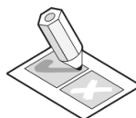
daily Scrum
