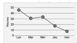
burndown chart
